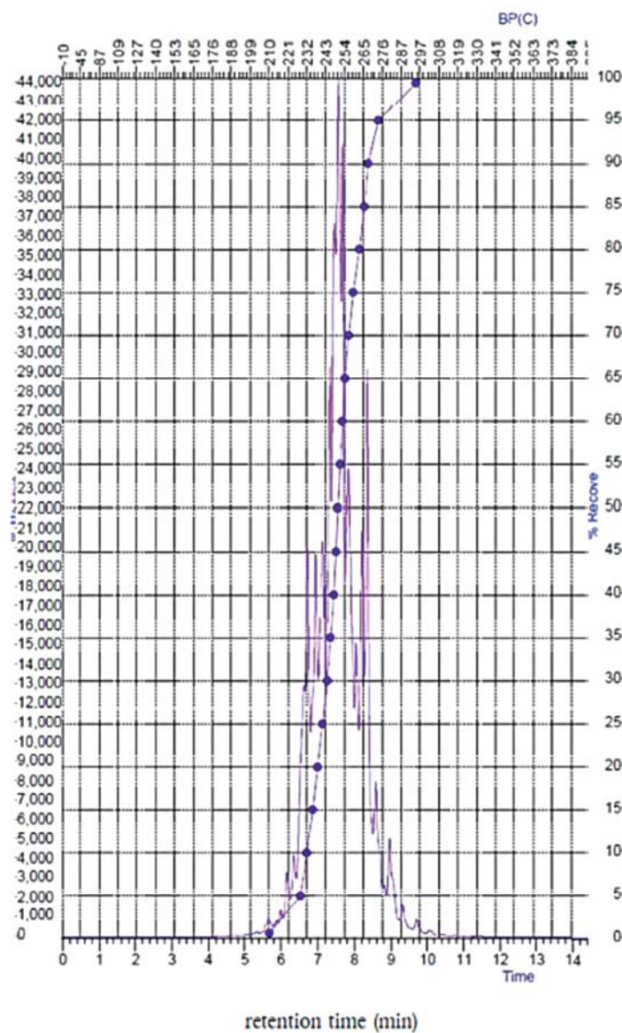
SIMDIS ASTM D 2887 extended correlation to ASTM D 86
