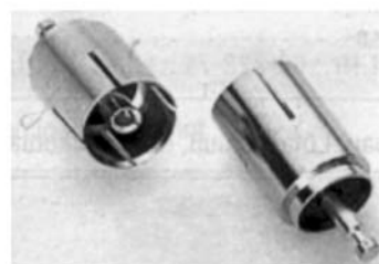
Figure 4 Coaxial socket
